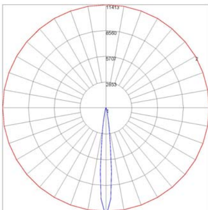
Optic Distribution: 10°
