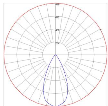
Optic Distribution: 60°
