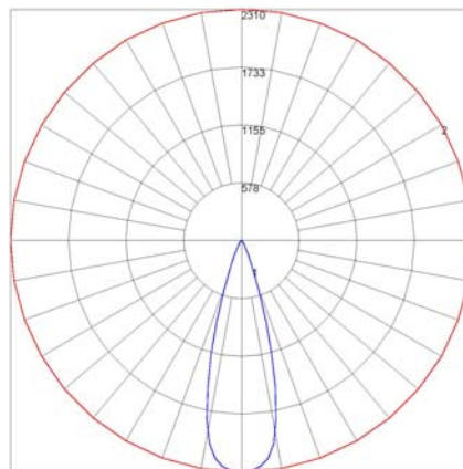
Optic Distribution: 30°
